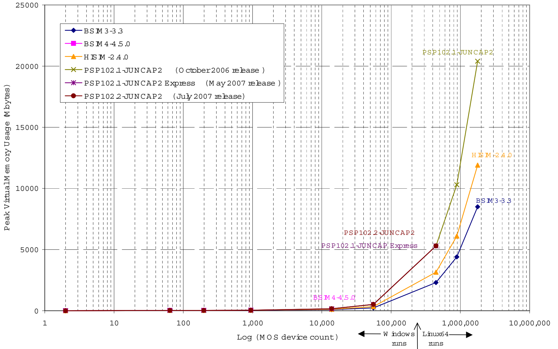
Silvaco 90nm Models /SmartSpice Peak VirtualMemory Usage /Circuits with no Parasitic Devices
