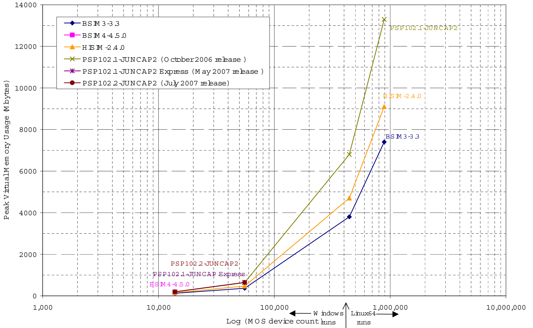
Silvaco 90nm Models / SmartSpice Peak Virtual Memory Usage / Circuits With Parasitic Devices
